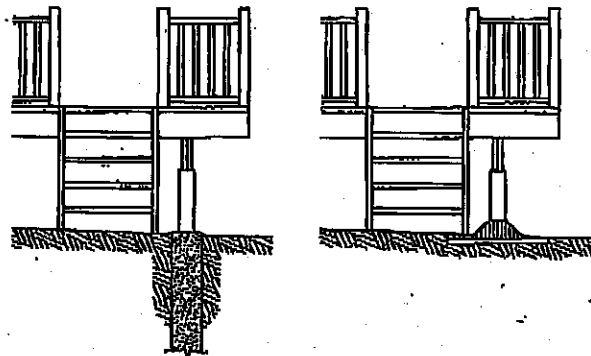
CONCRETE PILES
